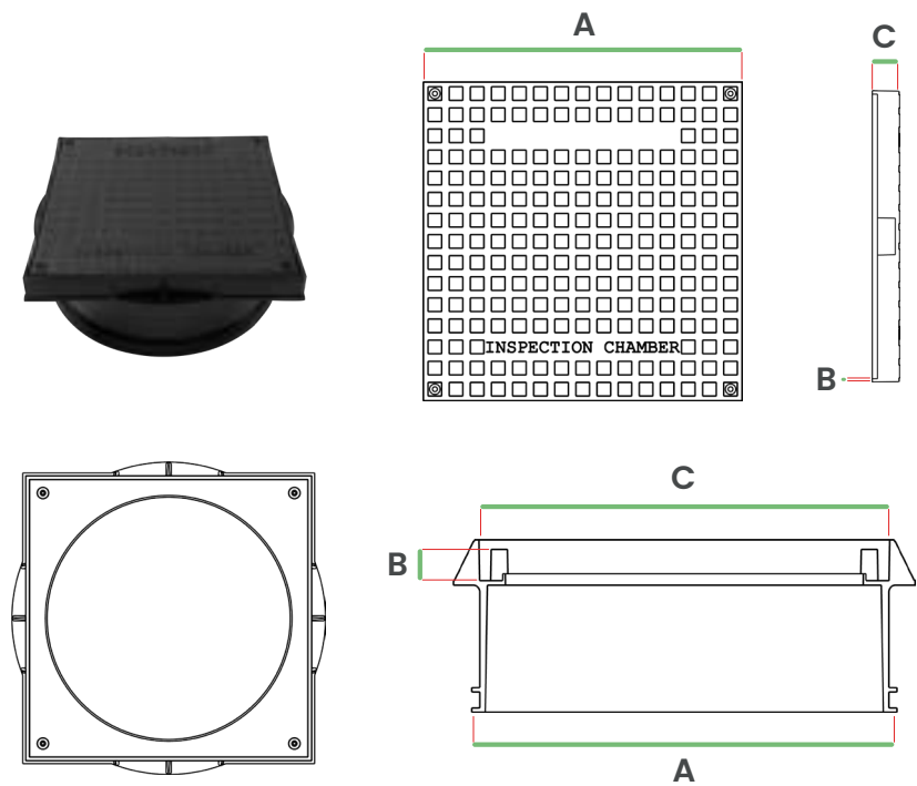
320mm Secured Square Cover & Frame 15KN [SCF320]
