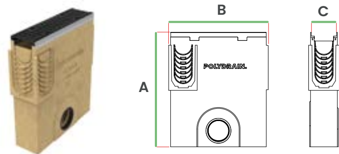
ProDrain 6mm Ductile Iron Safeheel Grating Sump Unit 150 [W] [PD15SU6D400]
